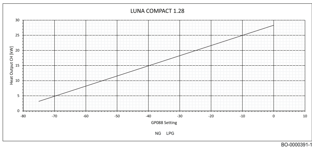
Obr.53 Graf pro LUNA COMPACT – 1.28
