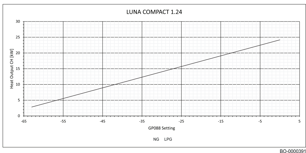
Obr.114 Graf pre LUNA COMPACT –1.24
